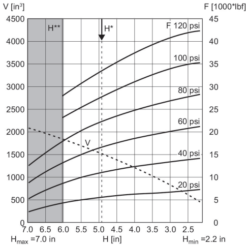
Diagramme force/course R432039310
