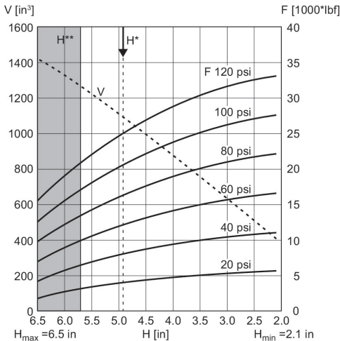
Diagramme force/course R432039308
