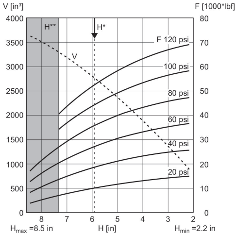
Diagramme force/course R432039313
