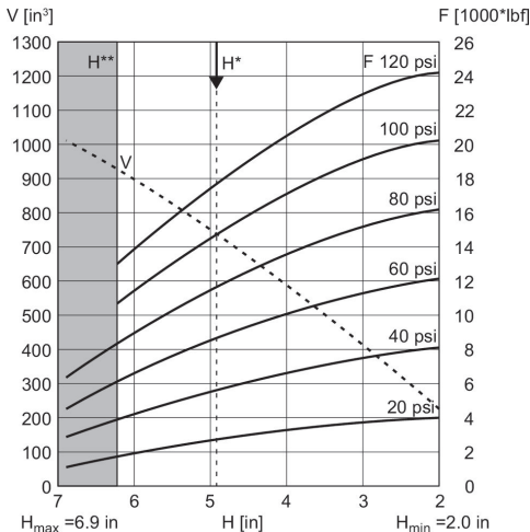
Diagramme force/course R432039303
