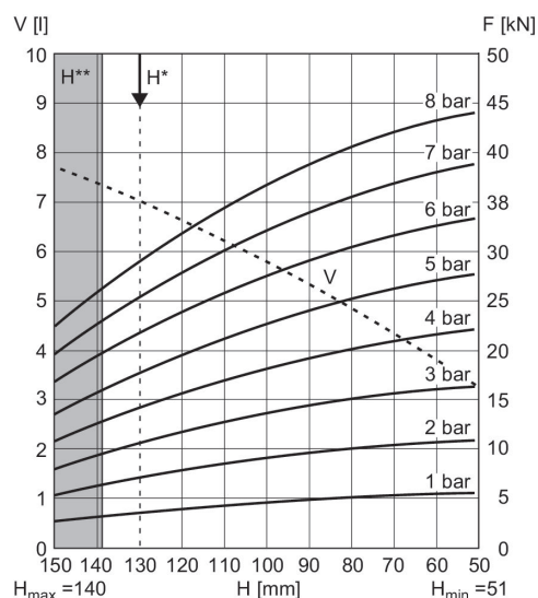
Diagramme force/course R412010219
