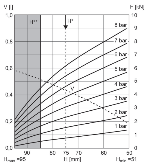
Diagramme force/course R412010215
