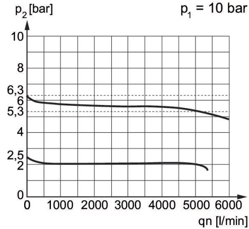
Flow rate characteristic ( p_2 : 0,5 - 8 bar)
