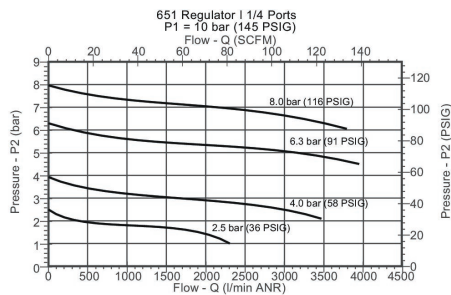
Flow diagram G 1/4
