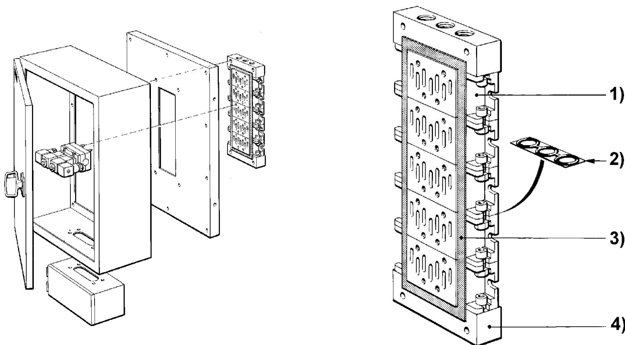
1) intermediate plate 2) intermediate plate gasket 3) sealing strip 4) end plate
