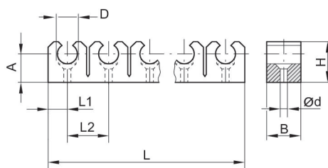
D = 4, 5, 6, 8 mm
